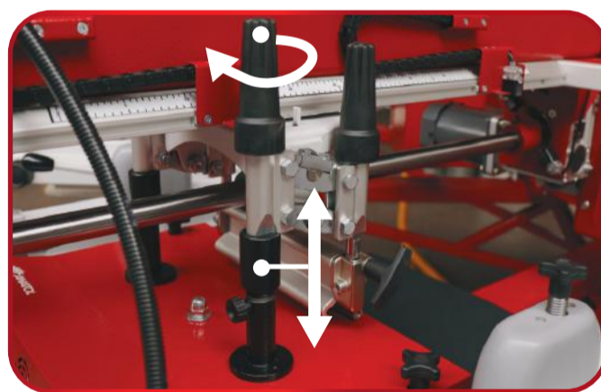
Mechanical depth adjustment
