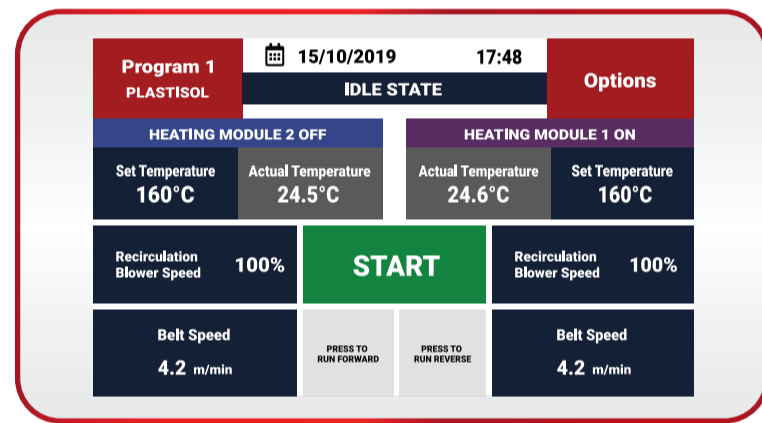
Color touchscreen control display
